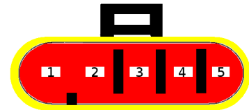
WBO2 (SSC5 female)
